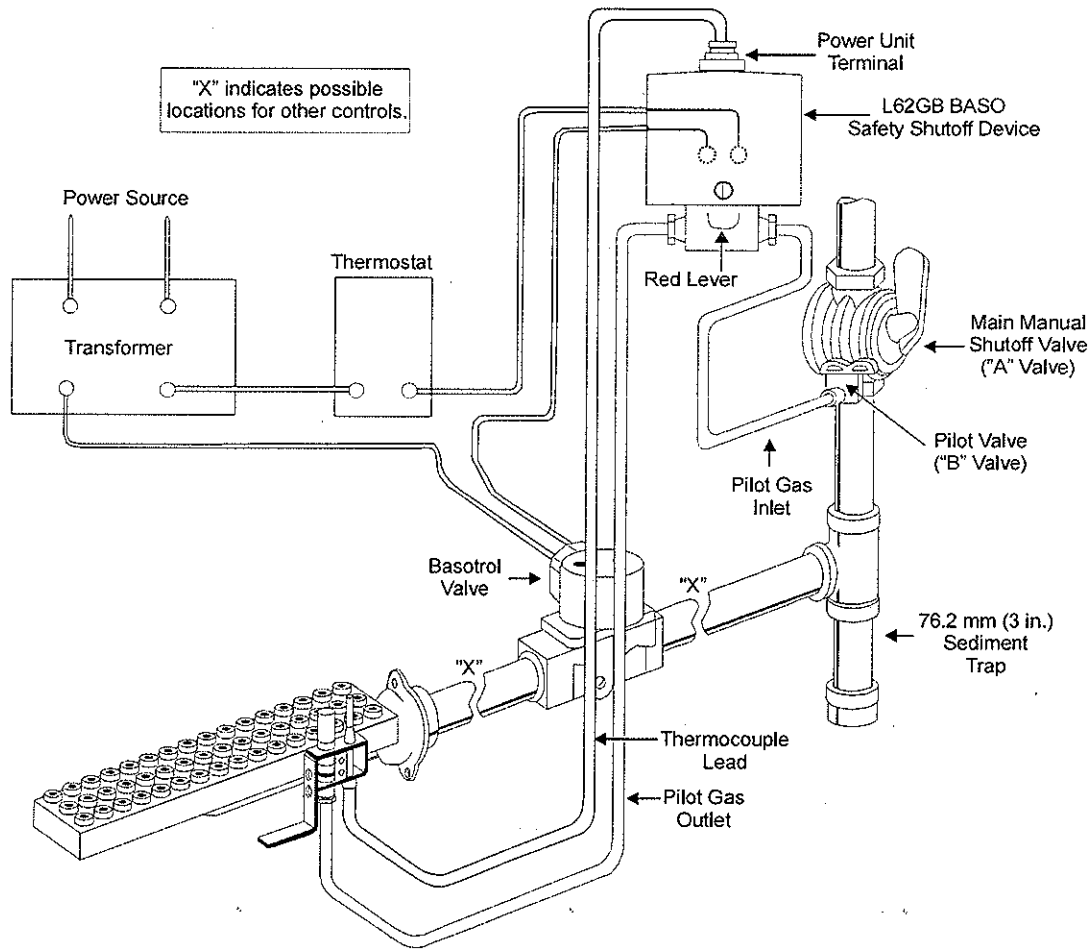
Figure 1: Typical L62GB Installation
