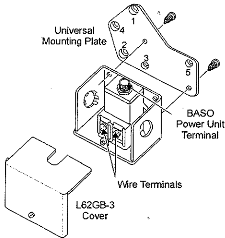
Figure 3: L62GB-3 Mounting
