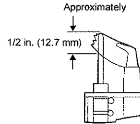
Figure 2: Flame Position
